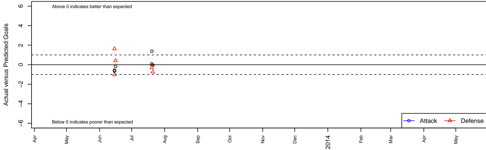
TSS Academy Weston B01 Dots are actual minus expected GF (blue circles) and GA (red triangles). Blue line is smoothed change in attack strength. Red is smoothed change in defense strength.
